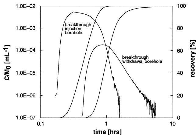
Fig. 5. 'Breakthrough injection bore hole': uranine concentration–time distribution (CTD) and recovery curves in injection bore hole ( P_i ); 'Breakthrough withdrawal bore hole': uranine BTC and recovery curves in withdrawal bore hole ( P_w ). Note small delay resulting in influence of BTC in P_w by CTD in P_i ; recovery curves shown at linear vertical axis, at right-hand side; shorter flow distance of 1.7 m; Run no. 75.
